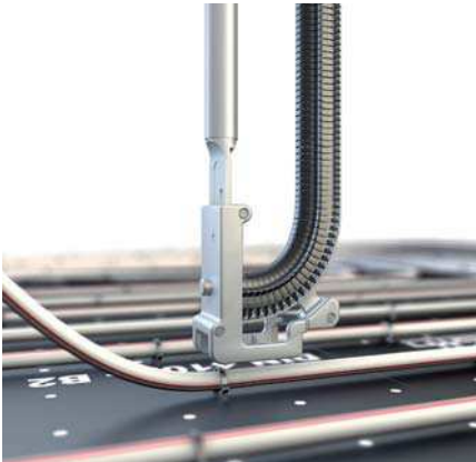
Roth Original-Tacker®-System
