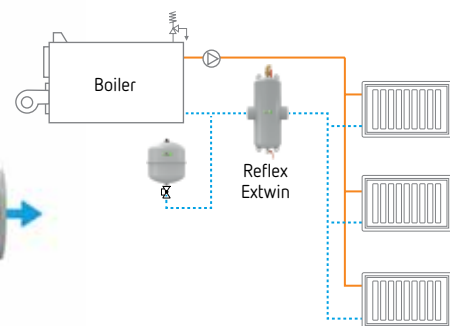
Extwin "Steel" system with combined micro-bubble dirt and sludge separation sketch
