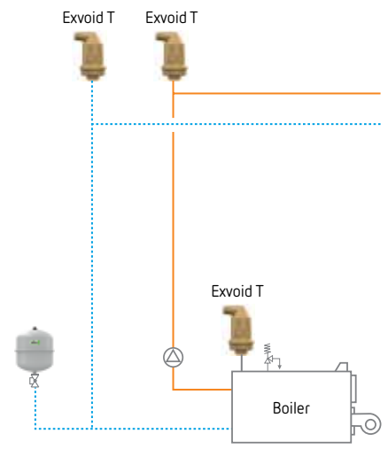
Exvoid T system air venting sketch
