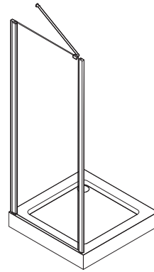
Side wall on the hinged side 1 × CSW1A90 (width 900 mm)
