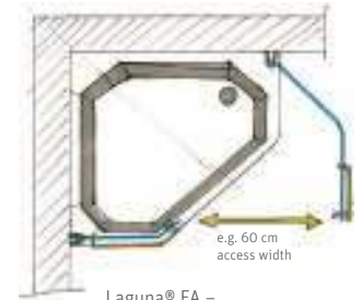
Laguna® FA – asymmetrical pentagonal shower
