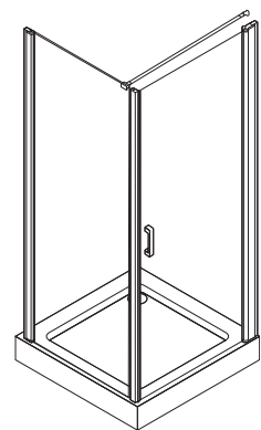
■ Corner shower 1 × CE290 (width 900 mm) + 1 × CSW1590 (width 900 mm)
