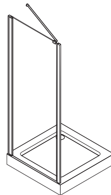
Side wall on the hinged side 1 × C5W1A90 (width 900 mm)
