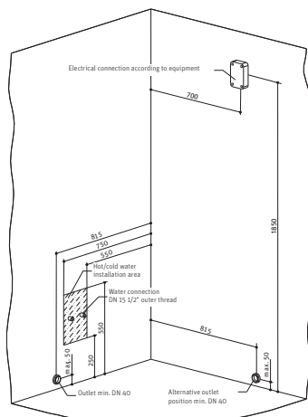
Installation sketch for Tempofit Corner and Round 920 x 920
