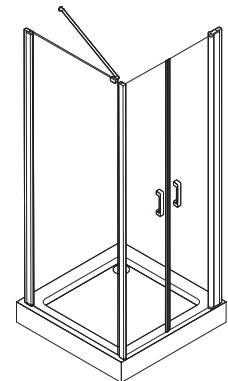
Corner shower 2 × CP245 (width 900 mm) + 1 × C5W1A90 (width 900 mm)
