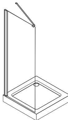
Side wall on the closure side 1 × CSW1590 (width 900 mm)
