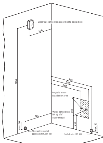
Installation sketch for Tempofit Corner 1020 x 755
