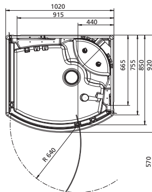
Swing door (r.) with side wall (l.)
