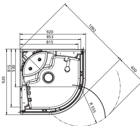
Swing door, 1 piece (r.)
