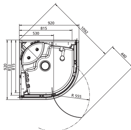
Swing door, 1 piece (l.)
