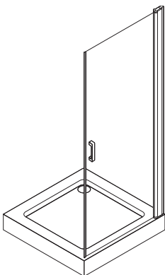
Corner door leaf without fixed element 1 × CE290 (width 900 mm)
