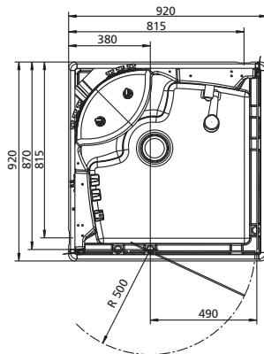
Swing door (l.) with side wall (r.)
