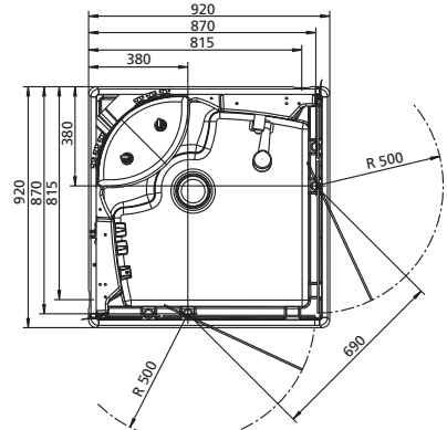
Swing door, 2 pieces
