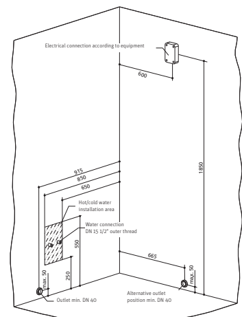
Installation sketch for Tempofit Corner 755 x 1020
